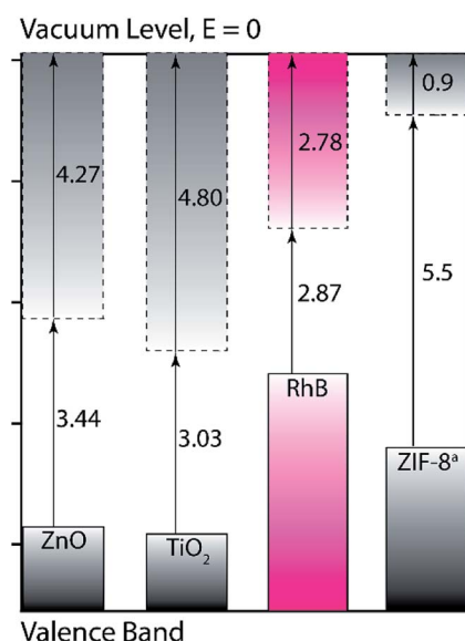
Scheme 2 Comparison of calculated electronic energy levels of RhB, ZIF-8, ZnO, and rutile \text{TiO}_2 (in eV respect to vacuum level). Dash and solid boxes represent conduction band and valence band, respectively. a Values were taken from DFT calculations with periodic boundary conditions. 64 The values for ZnO and \text{TiO}_2 are taken from previously reported DFT predicted bandgap. 70,71
