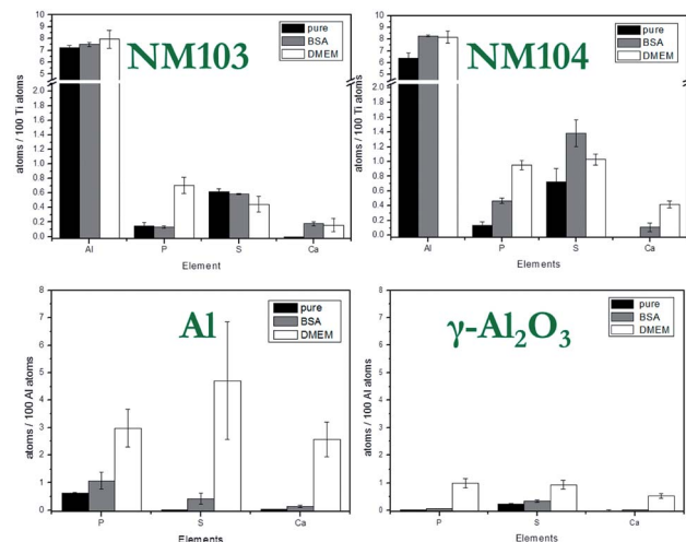
Fig. 8 IBM element analysis of NM103, NM104, Al and Al 2 O 3 NMs. NMs as purchased and diluted in water (pure), NMs with albumin corona in H 2 O (BSA) and NMs under cell exposure conditions (DMEM). The graph demonstrates the ratio of atoms of several elements compared to 100 atoms of titanium or aluminum.
