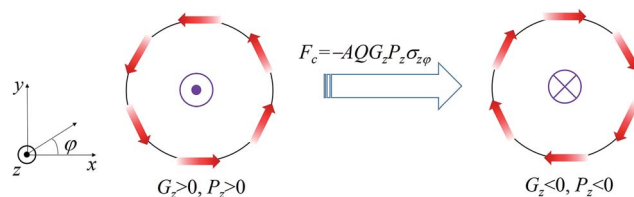
Fig. 9 Schematic of vortex switching in a ferroelectric nanoring based on the trilinear coupling between toroidization G_z , polarization component P_z , and shear stress \sigma_{\varphi z} .
