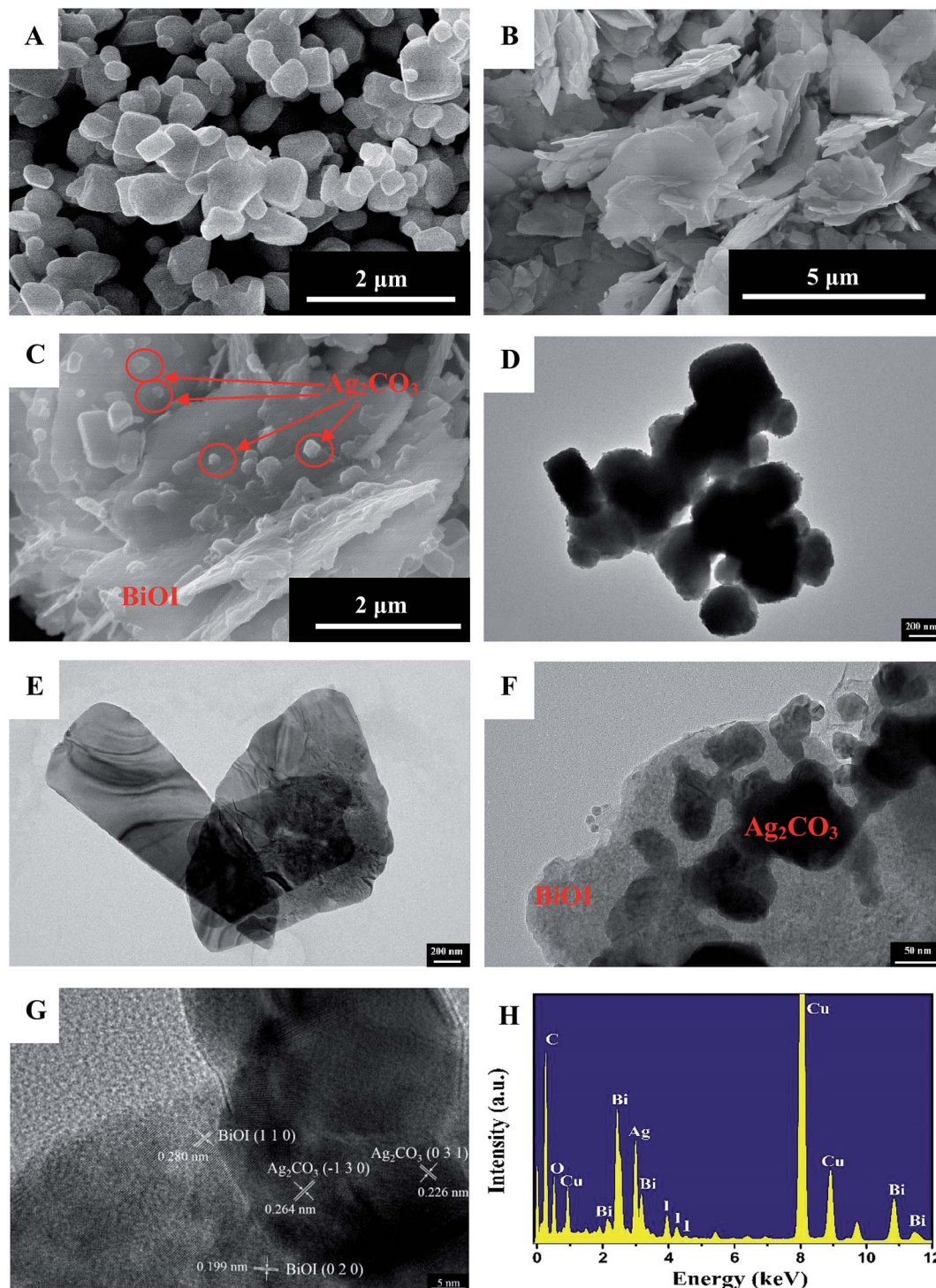
Fig. 4 The SEM images of (A) pure \text{Ag}_2\text{CO}_3 , (B) \text{BiOI} and (C) \text{BiOI}/\text{Ag}_2\text{CO}_3 (20 wt%) composite; the TEM images of (D) pure \text{Ag}_2\text{CO}_3 , (E) \text{BiOI} , (F) \text{BiOI}/\text{Ag}_2\text{CO}_3 (20 wt%) composite; (G) the HRTEM image and (H) EDX spectrum of \text{BiOI}/\text{Ag}_2\text{CO}_3 (20 wt%) composite.
