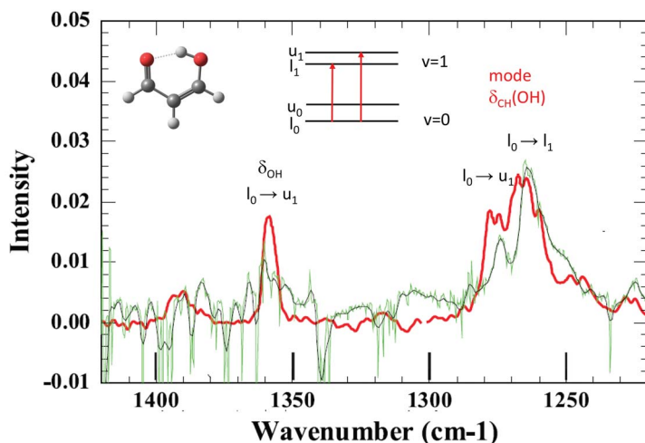
Fig. 3 Comparison between the spectrum of MA obtained by Suhm and co-workers in the gas phase (red line), from ref. 4, and the spectrum of MA in p H 2 (black lines) in the spectral range around the hybrid mode at ~1270 cm -1 (bending mode of the CH group – OH side). Only transitions from the lower level in the ground state ( l 0 ) can appear in p H 2 : l 0 → u 0 and l 0 → u 1 in the case of hybrid modes. The assignments are those of Lüttschwager et al. , ref. 4.
