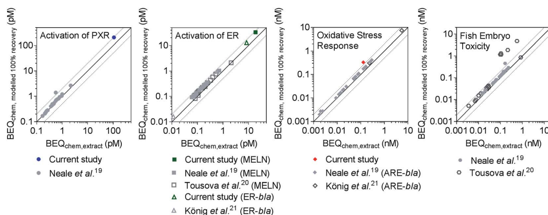
Fig. 3 Comparison of BEQ chem,extract and BEQ chem,modelled 100% recovery for activation of PXR, activation of ER (both ER GeneBLAzer (ER-bla) and MELN), oxidative stress response and fish embryo toxicity for the current study, Neale et al. , 19 König et al. 21 and Tousova et al. 20 The dotted lines indicate a factor of 2 difference between BEQ chem,extract and BEQ chem,modelled 100% recovery . NB: two different oxidative stress response assays based on the same endpoint were included, with AREc32 applied in the current study and ARE GeneBLAzer (ARE-bla) applied in Neale et al. 19 and König et al. 21
