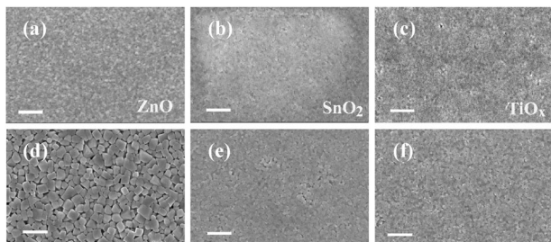
Fig. 3 SEM images of perovskite films deposited on ZnO, SnO 2 and TiO x substrates before (a–c) and after (d–f) vacuum-processing, respectively. The scale bar is 1 μm.
