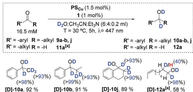
Scheme 5 Deuterium labelling studies of aromatic ketones ( 9a–b, j ), and aliphatic aldehydes ( 11a ). [a] 1 (6 mol%), \text{PS}_{\text{Cu}} (6 mol%), substrate (4.4 mM) in \text{D}_2\text{O} : \text{CH}_3\text{CN} : ^i\text{Pr}_2\text{EtN} (6 : 4 : 0.2 mL) irradiated (447 nm) for 24 h at -3^\circ\text{C} under \text{N}_2 . Isolated yields. Deuterium insertion analysed using NMR.
