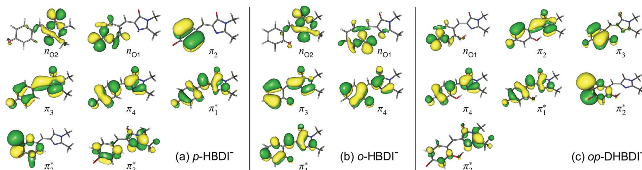
Fig. 5 Hartree–Fock (HF) orbitals of (a) p -HBDI − , (b) o -HBDI − and (c) op -DHBDI − used in the ADC(2)/aug-cc-pVDZ calculations. The HOMO is \pi_4 and the LUMO is \pi_1^* . The HF orbitals that were employed in the EOM-IP-CCSD calculations are very similar and therefore not shown.
