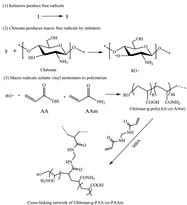
Fig. 1 General mechanism for radical graft polymerization of acrylamide and acrylic acid onto chitosan in the presence of MBA as cross-linker. Reproduced from ref. 16. Copyright (2004), with permission from Elsevier.
