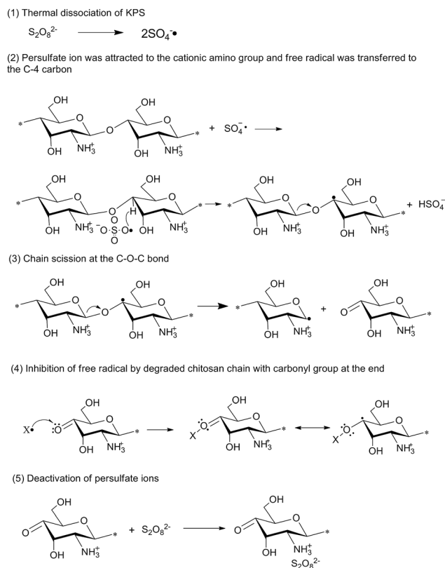
Fig. 2 The proposed mechanism for the degradation of chitosan by KPS free radical. Reproduced from ref. 59. Copyright (2006), with permission from Elsevier.
