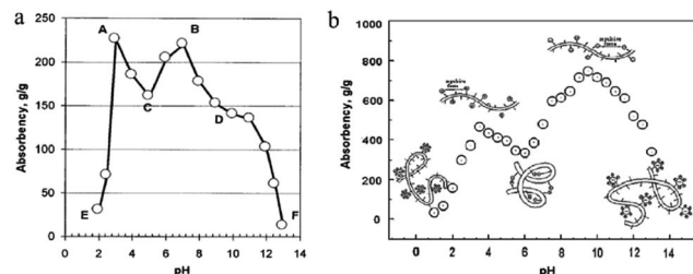
Fig. 5 Water-absorbency of superabsorbent hydrogel dependence on pH: (a) hydrolytic chitosan- g -polyacrylonitrile. Reproduced from ref. 38. Copyright (2003), with permission from Wiley-VCH. And (b) carboxymethyl chitosan- g -polyacrylic acid- co -dimethyldiallylammonium chloride. Reproduced from ref. 52. Copyright (2010), with permission from Elsevier.
