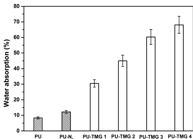
Fig. 8 Water absorption properties of PU, PU- \text{N}_3 , PU-TMG 1 (wt% = 0.6%), PU-TMG 2 (wt% = 1.0%), PU-TMG 3 (wt% = 2.1%), and PU-TMG 4 (wt% = 5.5%) at room temperature for 72 hours.
