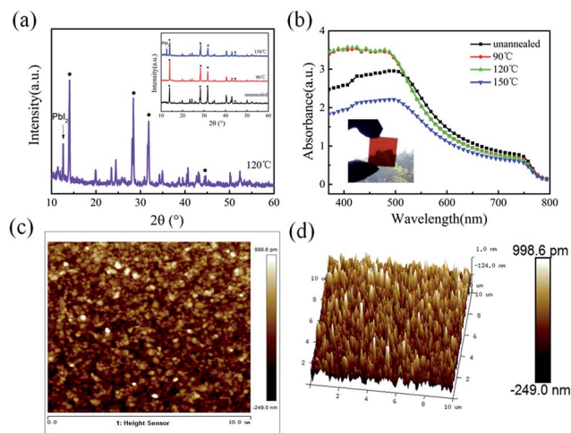
Fig. 3 (a) XRD patterns and (b) the absorption spectra of the \text{CH}_3\text{NH}_3\text{PbI}_3 thin films after annealing at different temperature, respectively. (c) 2D, (d) 3D AFM characterizations of the LFCVD \text{CH}_3\text{NH}_3\text{PbI}_3 thin film after annealing at 120\text{ }^{\circ}\text{C} on the FTO/c- \text{TiO}_2 substrate.
