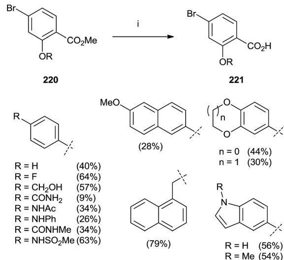
Scheme 38 Reagents and conditions: (i) 1: boronic acid, Pd(PPh_3)_4 , Na_2CO_3 , DME/EtOH , H_2O , MW (110 °C), 10 min. (ii) LiOH , MeOH/THF , MW (110 °C), 12 min.
