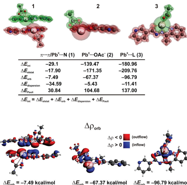
Fig. 9 (Top) Cluster models of [PbL(OAc)] 2 together with the fragmentation patterns 1–3 applied in the ETS-NOCV analysis. (Bottom) The overall deformation densities Δρ orb of 1–3 with the corresponding energies ΔE orb .
