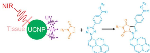
Fig. 15 NIR photo-coupling reaction based on nitrile imine-mediated tetrazole-ene cycloadditions in the presence of UCNPs. This type of photoreaction at interfaces still awaits exploration.
