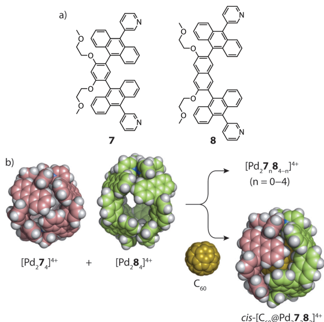
Fig. 6 (a) Short (7) and long (8) anthracene-functionalized ligands; (b) C 60 -templated integrative self-sorting of cages [Pd 2 7 4 ] 4+ and [Pd 2 8 4 ] 4+ to give the heteroleptic host-guest complex cis -[C 60 @Pd 2 7.8 2 ] 4+ . Reproduced with permission from ref. 54.
