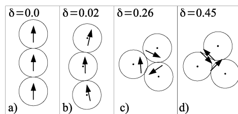
Fig. 2 (a–d) Ground state configurations of three particles.
