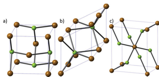
Fig. 6 The three major phases of iron selenide: (a) \alpha -FeSe, (b) achavalite and (c) ferroselite ( \text{FeSe}_2 ). Brown = Fe, green = Se.
