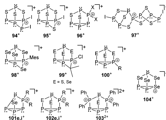
Fig. 17 Selected cationic polyphosphorus–chalcogen cages 94 + – 103 2+ ( E = S , Se ) comprising bonding motif J ; cation 104 + has been included since it represents the first binary SeP -cation and is related to the other cations.
