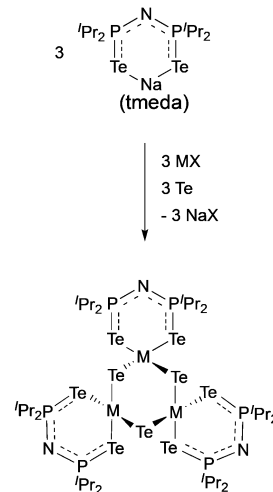
Scheme 3 General synthesis of [\text{Ga}(\mu\text{-Te})\{\text{N}(\text{TeP}^i\text{Pr}_2)_2\}_3]_3 ( \text{M} = \text{Ga} , \text{X} = \text{I} ) and [\text{In}(\mu\text{-Te})\{\text{N}(\text{TeP}^i\text{Pr}_2)_2\}_3]_3 ( \text{M} = \text{In} , \text{X} = \text{Cl} ).
