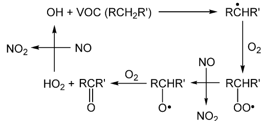
Scheme 2 Generation of \text{NO}_2 during typical oxidation of volatile organic compounds (VOC) by \text{OH} .
