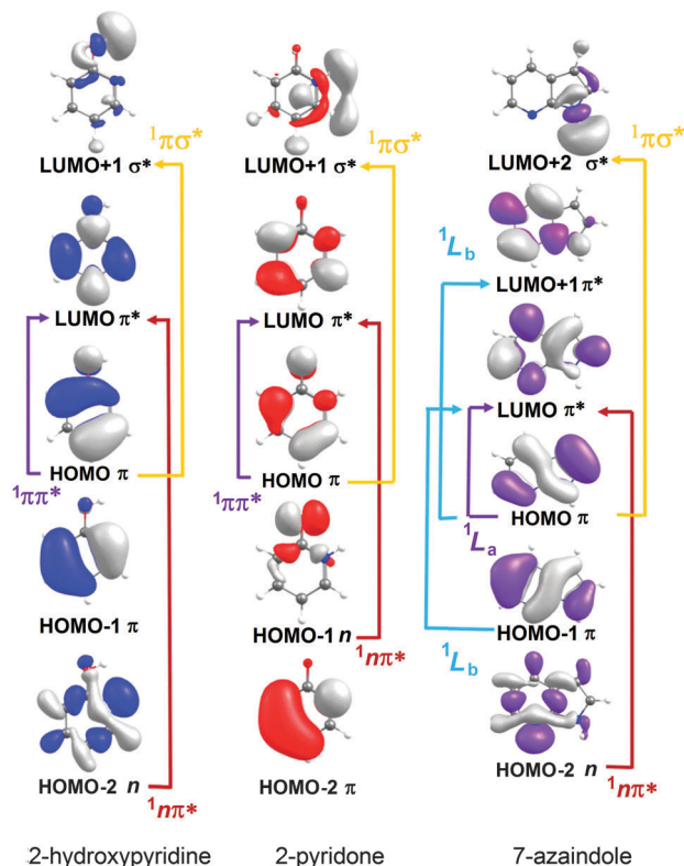
Fig. 7 Dominant orbital promotions involved in forming the first few singlet excited states of 2-hydroxypyridine, 2-pyridone and 7-azaindoles.
