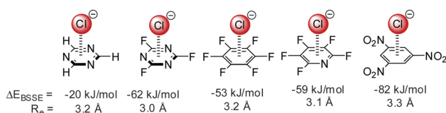
Fig. 2 Interaction energy with basis set superposition error correction ( E_{\text{BSSSE}} ) and equilibrium distances ( R_e ) of selected anion- \pi complexes from the MP2/6-31++G** level of theory. 7,15,16
