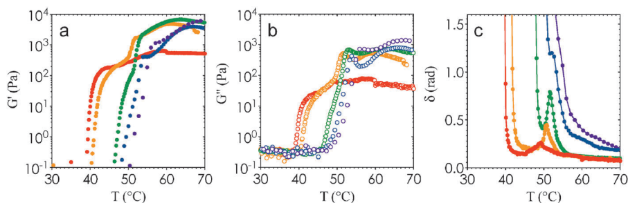
Fig. 6 Effect of heating rate on viscoelastic properties of gels. The values of (a) G' , (b) G'' , and (c) \delta are plotted as a function of T for nanoemulsions ( \phi = 0.25 ) heated at a rate of 0.5 °C \text{min}^{-1} (red), 1 °C \text{min}^{-1} (orange), 2 °C \text{min}^{-1} (green), 5 °C \text{min}^{-1} (blue), and 10 °C \text{min}^{-1} (purple).
