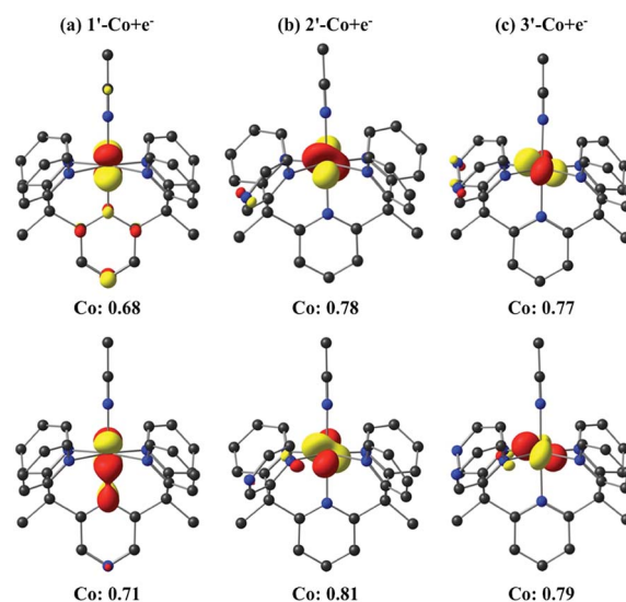
Fig. 9 Isosurface (0.07 au) plots of the canonical highest occupied molecular orbitals (HOMOs, top) and β-spin localized orbitals (bottom) for 1'-Co + e − , 2'-Co + e − and 3'-Co + e − ( S = 1). The Löwdin population analyses are given for cobalt.
