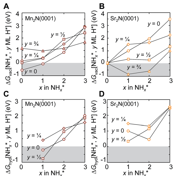
Fig. 3 Free energy diagrams for (A and B) forming 1/4 ML v_N yielding 1/4 ML NH_x^* and (C and D) hydrogenating NH_{x-1}^* to NH_x^* and y ML H^* at Mn_2N(0001) (A and C) and Sr_2N(0001) (B and D) at 25^\circ C and 1 bar. Lines are a guide only. The shaded regions mark energetically favourable surface reactions.
