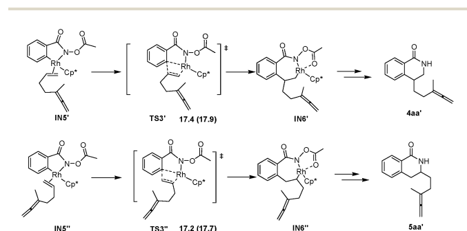
Scheme 9 The activation free energies of forming 4aa' and 5aa' ( \Delta G_{\text{sol}} ( \Delta G_{298\text{ K}} )).
