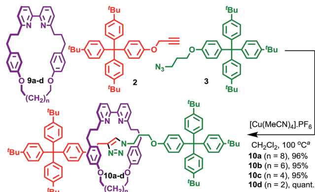
Scheme 2 Selective synthesis of [2]rotaxanes 10 with macrocycles 9 . a 1 equiv. 9 , 1.2 equiv. each 2 and 3 , 0.96 equiv. [Cu(MeCN) 4 ] 2 ·PF 6 , 50 mM conc. of 9 , CH 2 Cl 2 100 °C (μW), 15 min. The ratio of [2] : [3] rotaxane was >98 : <2 in all cases.
