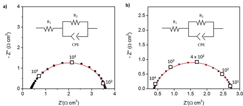
Fig. 6 Symmetric cell impedance measurements of 30 wt% Pt-CNT based electrodes prepared by (a) strategy 1 in which Pt-CNT bearing and CDP bearing solutions were electro sprayed sequentially, and (b) strategy 2 in which a single Pt-CNT and CDP bearing solution was sprayed. In (a), the Pt loading and utilization are 4.2 \times 10^{-3} \text{ mg cm}^{-2} Pt and 64 \text{ S mg}^{-1} , respectively, whereas in (b) they are 5.1 \times 10^{-3} \text{ mg cm}^{-2} Pt and 86 \text{ S mg}^{-1} . Measurements are performed at 240^\circ \text{C} in a dynamic atmosphere of 0.4 \text{ atm H}_2\text{O} and balance \text{H}_2 supplied at a gas velocity of 6 \text{ cm min}^{-1} and spectra are taken after 4 hours (insets: equivalent circuit used for fitting).
