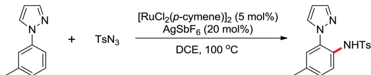
Scheme 164 Ru(II)-catalyzed C–H amidations of heteroaryl arenes.
