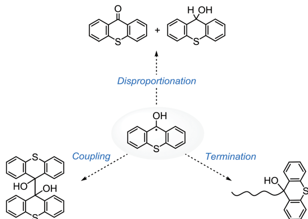
Scheme 4 Possible reactions of thioxanthy ketyl radicals.
