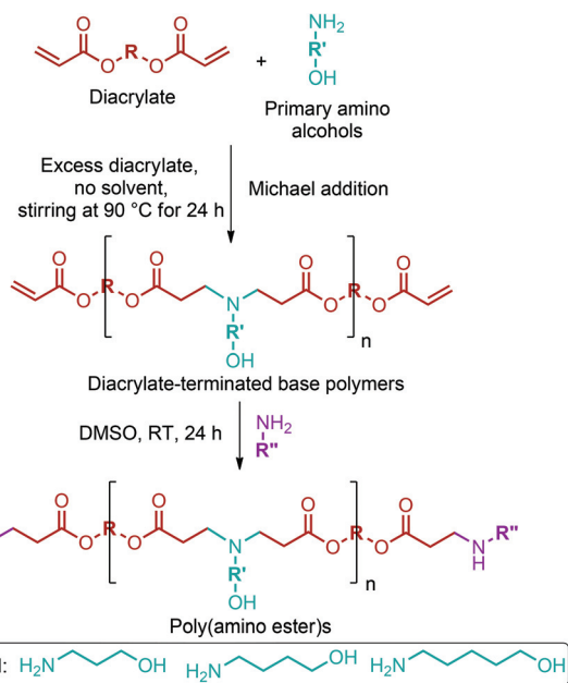
Fig. 18 Synthesis of the poly(β-amino ester) library. Adapted from ref. 306.
