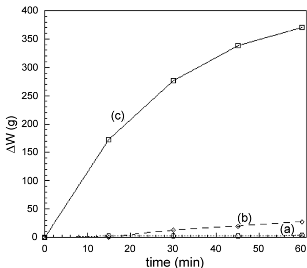
Fig. 11 Weight loss of calibrated copper wires (500 mg, Ø = 0.3 mm) in the given time (minutes) by treatment with NH 3 /(NH 4 ) 2 SO 4 ( 4.4 \times 10^{-3} M and 6.0 \times 10^{-4} M, respectively): (a) without additions (---○---); (b) with 30 mL NaOH 1.5 M/I 2 (5 g) solution (---◇---); and (c) 2.7 mL H 2 O 2 35% (---□---) additions.
