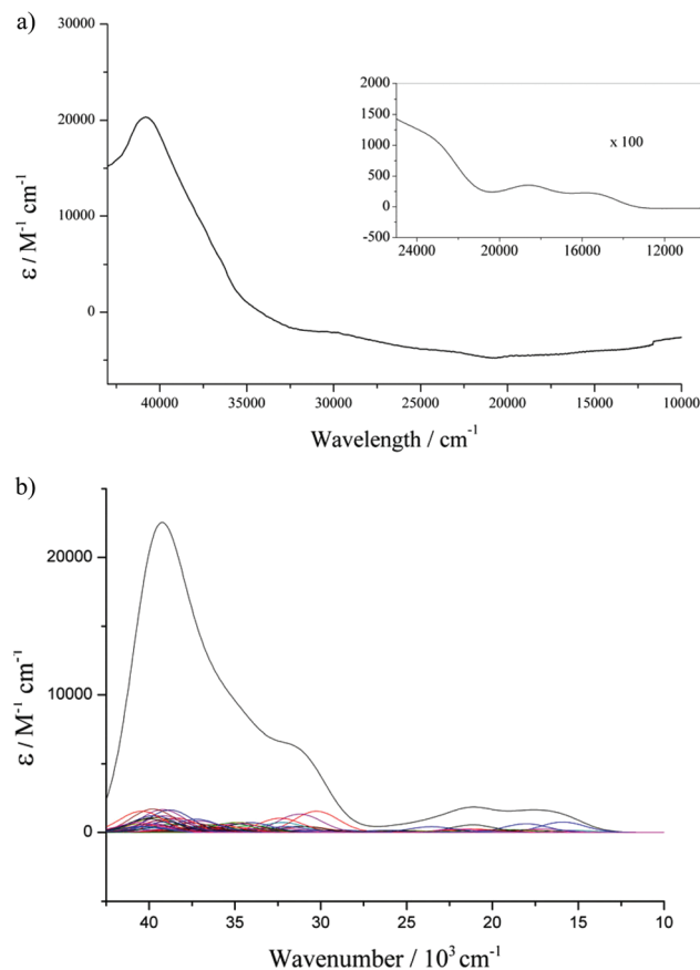
Fig. 8 (a) UV-vis spectra of 2Cl at 1.25 mM and 0.0125 mM (insert) in THF solution. (b) Predicted UV-vis spectrum of 2Cl showing the individual electronic transitions and the combined total in the gas phase.
