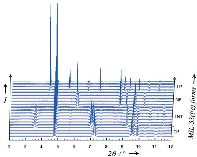
Fig. 3 Adsorption of CO 2 on MIL-53(Fe) followed by X-ray powder diffraction. Four different phases can be identified depending on the pressure and/or temperature (anhydrous CP, INT, NP and LP forms).
