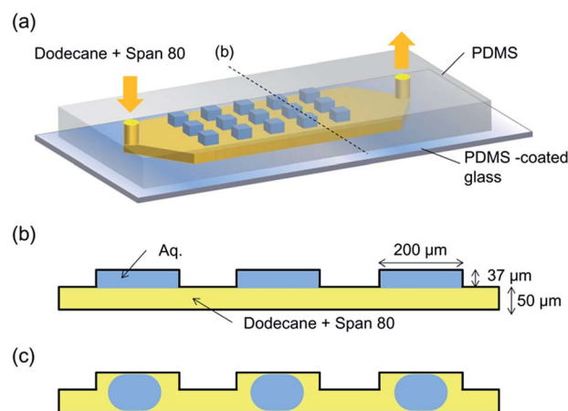
Fig. 2 A microfluidic device for microdroplet formation. (a) Overview of the device. A cross-sectional view of the microchannel shortly after the aqueous solutions were chambered (b), and when the solutions were exposed to a flow of dodecane containing Span 80 (c).
