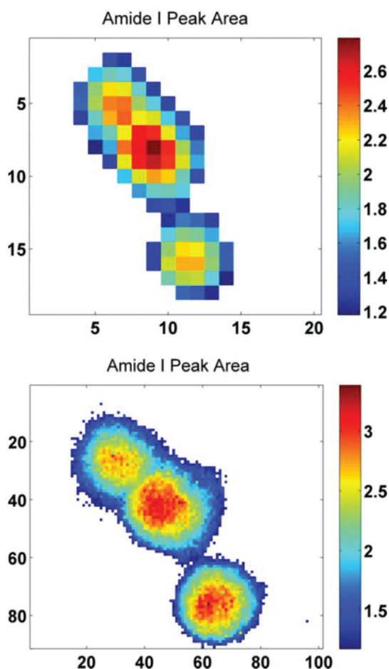
Fig. 4 (top–bottom) Photo-micrograph taken with a 40x objective, at a pixel resolution of 0.27 μm. The amide I integrated peak area maps are presented for the raw spectral images acquired with normal and high magnification imaging modes respectively. The axes reflect the number of pixels, covering an area equivalent to ~100 × 111 μm.
