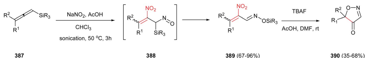
Scheme 133 Synthesis of isoxazolidinone derivatives from \alpha -nitro- \alpha,\beta -unsaturated silyloximes.
