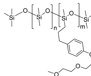
Scheme 46 Glyme-substituted polysiloxane stationary phase.
