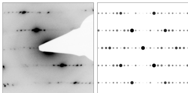
Fig. 8 Experimental SAED pattern (zone axis <110>, left) of a crystal from a bulk sample of Ge 1.3 Sn 0.7 Sb 2 Te 5 and the corresponding calculated one (right) based on the structure model from Ge 1.3 Sn 0.7 Sb 2 Te 5 .
