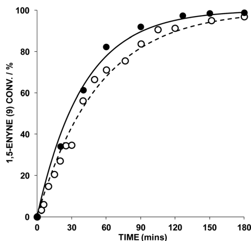
Fig. 2 Effect of AgOTf equivalents relative to AuBr 2 ( N -TFS)( I t Pe) in 1,5-ene cycloisomerisation of 9 (key: ● = 2 mol% AgOTf; ○ = 1 mol% AgOTf). Other details: [9] = 0.2 M, DCE, 1 mol% Au cat., 25 °C; 1,5-ene conversion was monitored by HRGC – each sample point was quenched by addition of N( n -Bu) 4 Br. The kinetic curves were fitted using Dynafit™.
