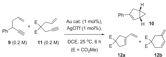
Scheme 3 Competition experiment of a 1,5-enyne 9 and 1,6-enyne 11 . Product 10 derives from 9 and products 12a and 12b from 11 . The kinetic profiles are shown in Fig. 6 and product distributions of 12a : 12b shown in Fig. 7.
