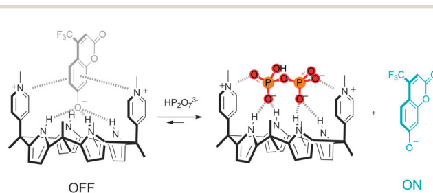
Scheme 3 Proposed Fluorescent Dye Displacement Assay (FDFA) detection of pyrophosphate anion by 45 .
