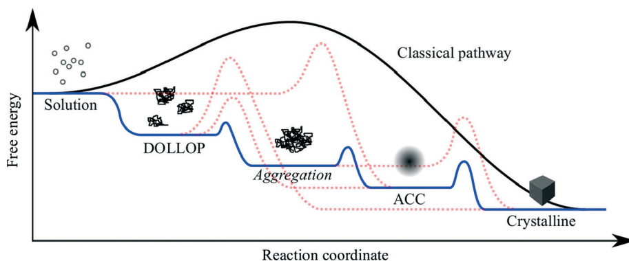
Fig. 1 Schematic showing the free energy variation for a variety of possible pathways for crystallisation from ions in solution. DOLLOP (Dynamically Ordered Liquid-Like Oxyanion Polymer) refers to the prenucleation clusters identified in ref. 3, (image courtesy of R. Darkins).
