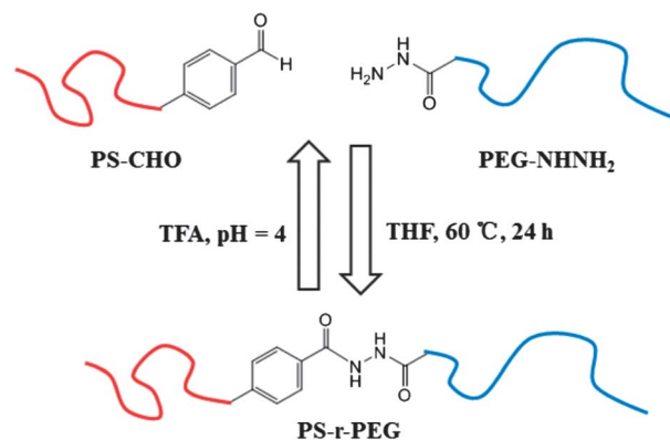
Fig. 2 Dynamic properties of PS- r -PEG. 44
