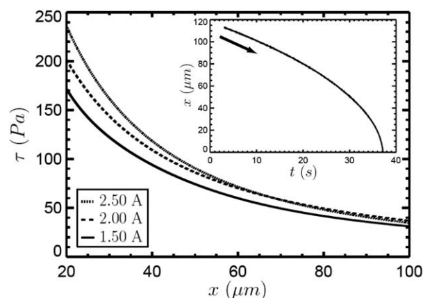
Fig. 2 Calibration curves for the stress applied by the magnetic tweezers as a function of the distance from the tip. Results for I = 1.50 A, 2.00 A, and 2.50 A are shown. The stress increases as the tip is approached and stresses up to about 230 Pa are accessible close to the tip. For x < 20 µm, the computed stress values are highly sensitive to the order of the polynomial fit to trajectory data. The stress exhibits only weak dependence on current, suggesting that either the core or the probe particles are approaching magnetic saturation. The inset shows a typical probe trajectory in the Newtonian calibration fluid, which has a kinematic viscosity of \nu = 30\,000 cSt ( \eta = 29.5 Pa s).
