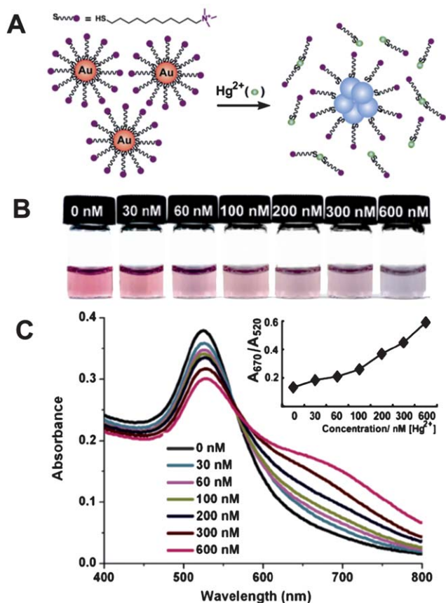
Fig. 1 Colorimetric detection of Hg 2+ based on the abstraction of quaternary ammonium group-terminated thiols from the surfaces of AuNPs. (A) The proposed mechanism for the Hg 2+ -induced colorimetric response of QA-AuNPs. (B) Light irradiation-assisted detection of Hg 2+ with the color change upon the increase of concentrations of Hg 2+ from left to right. (C) Absorbance response for (B). Inset: A_{670}/A_{520} vs. Hg 2+ concentrations. The irradiation time was 30 s, the pH value of the solutions was 1.0. Reproduced with permission from ref. 46. Copyright 2010, ACS.
