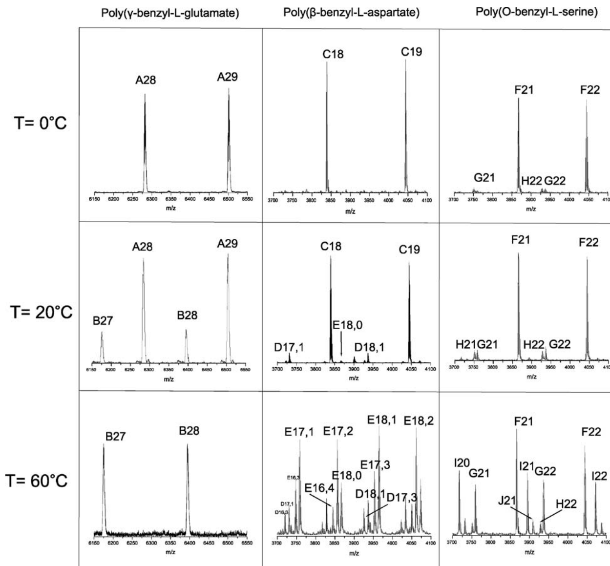
Fig. 1 MALDI-ToF-MS results of PBLG, PBLA and PBLs obtained at different temperatures. Letters in peak assignments refer to structures shown in Fig. 2; numbers denote the degree of polymerization. For the poly( \beta -benzyl-L-aspartate) the first number refers to the \beta -benzyl-L-aspartate units and the second number to the anhydrides units in the formed copolymers. All samples were measured with potassium trifluoroacetic acid (KTFA).
