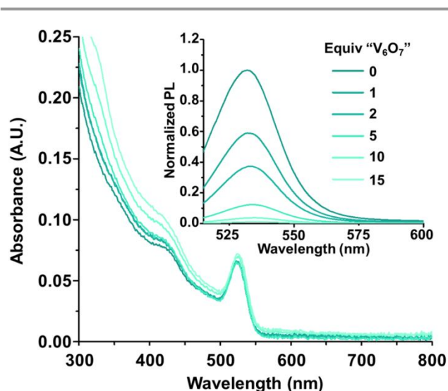
Figure 2. The absorbance and photoluminescence (inset) spectra of CdSe-TOP with varying equivalents of [V_6O_7(OC_2H_5)_{12}]^{-1} ("V 6 O 7 "). All samples contained 1 \mu M CdSe with 0-15 equivalents of [V_6O_7(OC_2H_5)_{12}]^{-1} in dichloromethane and the photoluminescence was normalized to the absorbance at the excitation wavelength (500 nm).
