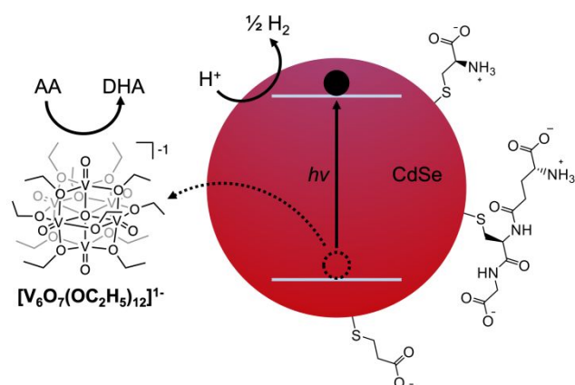
Figure 1. Illustration of the general photocatalytic scheme. Upon excitation by visible light, the electron reduces protons at the surface of the dot, while the hole is extracted by a POV-alkoxide cluster. Ascorbic acid is used to regenerate the reduced form of the cluster in solution. Capping ligands were chosen to promote solubility in aqueous solutions, and include cysteine (top), glutathione (middle), and 3-mercaptopropionic acid (bottom).
