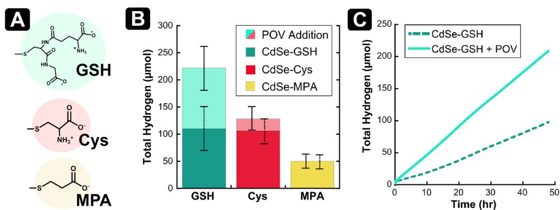
Figure 3. A) Structures of the capping ligands used on the surface of CdSe; B) Total H 2 evolution after 48 hours from CdSe-GSH, CdSe-Cys, and CdSe-MPA in the presence of 0.5 M ascorbic acid, in a 1:1 EtOH:H 2 O mixture, being irradiated by 530-nm light at 15 °C. Upon addition of 100 μM [V 6 O 7 (OC 2 H 5 ) 12 ] -1 , the positive change in total H 2 production for CdSe-GSH and CdSe-Cys is shown (n = 3); C) Representative trials of H 2 evolution over time for the CdSe-GSH H 2 evolution system described in B, showing improvement in the presence of [V 6 O 7 (OC 2 H 5 ) 12 ] -1 .
