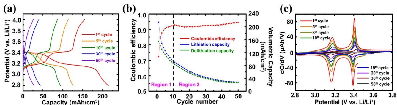
Figure 3. Electrochemical tests of V_2O_5 thin films. (a) Galvanostatic discharge/charge profiles measured during 50 cycles between 4.0 – 2.8 V vs. Li/Li^+ at a current density of 5.92 \mu A/cm^2 (0.2 C). (b) Corresponding coulombic efficiency and volumetric capacities. (c) Corresponding differential capacity curve at selected cycles.
