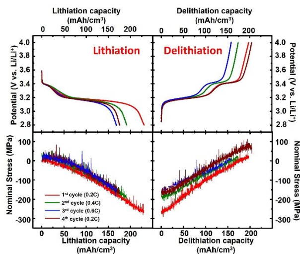
Figure 6. Potential and corresponding stress response during 4 cycles of a V_2O_5 thin film between 4.0 – 2.8 V vs. \text{Li}/\text{Li}^+ at varying current densities of 5.92 \mu\text{A}/\text{cm}^2 (0.2 C), 11.83 \mu\text{A}/\text{cm}^2 (0.4 C), 17.75 \mu\text{A}/\text{cm}^2 (0.6 C), and 5.92 \mu\text{A}/\text{cm}^2 (0.2 C).
