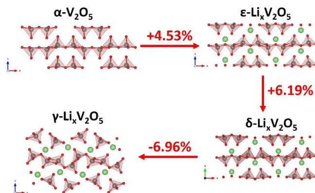
Figure 2. Crystal structures of various phases during lithiation of V 2 O 5 : \alpha -V 2 O 5 , \epsilon -Li x V 2 O 5 , \delta -Li x V 2 O 5 , and \gamma -Li x V 2 O 5 , and the corresponding volume expansion during each phase transformation.
