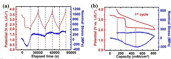
Figure 7. Potential and corresponding stress response during 3 galvanostatic cycles of a V_2O_5 thin between 4.0 – 2.0 V vs. \text{Li}/\text{Li}^+ at a current density of 5.92 \mu\text{A}/\text{cm}^2 (0.2 C). (b) Enlarged view of the first cycle.
