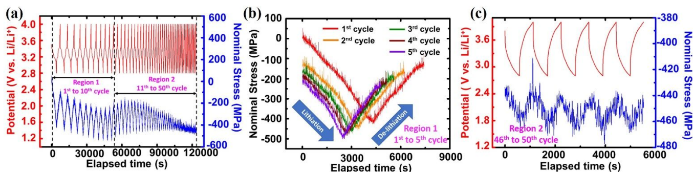
Figure 5 (a) Potential and corresponding stress response during 50 galvanostatic cycles of a V_2O_5 thin film between 4.0 – 2.8 V vs. Li/Li^+ at a current density of 5.92 \mu A/cm^2 (0.2 C). (b) Enlarged view of stress response during cycles 1-5. (c) Enlarged view of potential and corresponding stress response during cycles 46-50.
