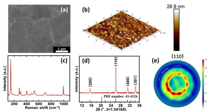
Figure 1. Surface morphology and structural characterization of V 2 O 5 thin films: (a) SEM image, (b) AFM image, (c) Raman spectroscopy, (d) X-ray diffraction pattern of as-deposited film on a stainless steel substrate, and (e) corresponding pole figure of V 2 O 5 thin film, indicating high texture in the (110) direction.
