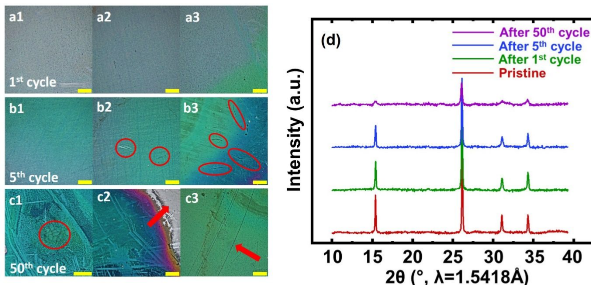
Figure 4. Optical microscopy images of V_2O_5 thin films after galvanostatic cycling between 4.0 – 2.8 V vs. Li/Li^+ at a current density of 5.92 \mu A/cm^2 (0.2 C). The scale bar in the figures indicates 300 \mu m . (a1-a3) Optical images of V_2O_5 thin film after 1 cycle, (b1-b3) after 5 cycles, and (c1-c3) after 50 cycles. (d) Evolution of XRD patterns of a V_2O_5 thin film during cycling.
