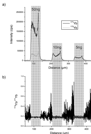
Fig. 2 LA-ICP-MS analysis of gel electrophoresis spots containing 50, 10 and 5 ng of MeCAT(Yb)-IA labeled HSA spiked with isotopically-enriched MeCAT( 171 Yb)-IA labeled HSA in a proportion 1:2: a) Signal intensities of isotopes 171 Yb and 172 Yb. b) Isotope ratio 172 Yb/ 171 Yb (reproduced from Ref. 8 with permission from the Royal Society of Chemistry).
